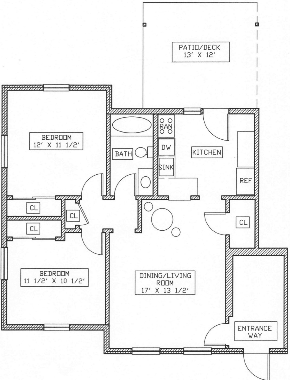
TWO BEDROOM: FIRST FLOOR ~ AREA PER UNIT: 780 & 794 SQ. FT.
